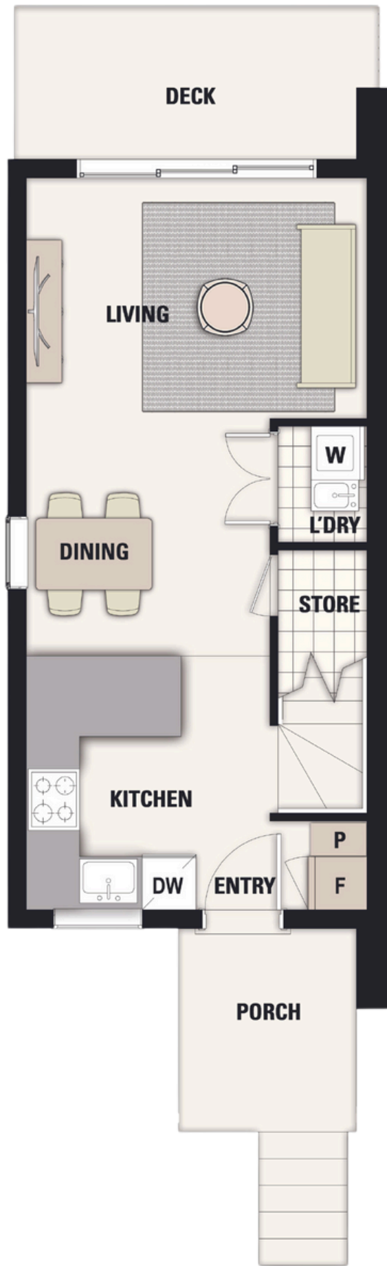
GROUND FLOOR
