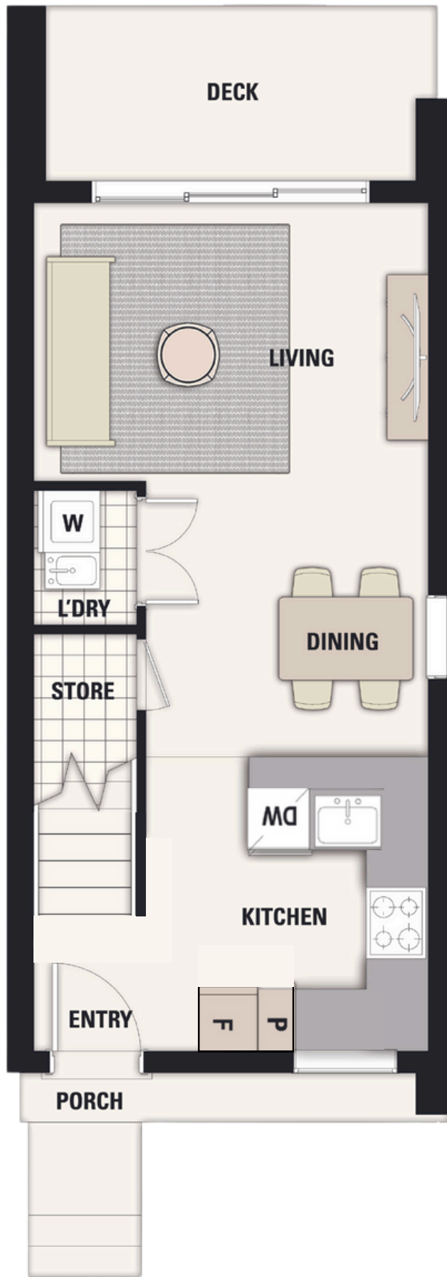
GROUND FLOOR
